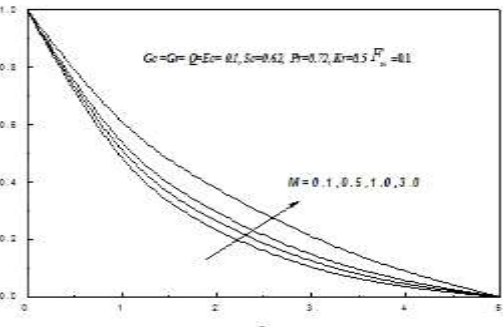
Fig. 18: Effect of the magnetic parameter ( M ) on concentration profiles.
