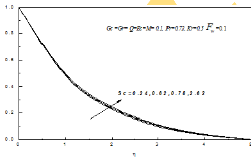
Fig. 13: Effect of the Schmidt number ( Sc ) on temperature profiles
