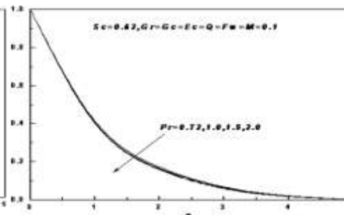
Fig. 8: Effect of the Prandtl number ( Pr ) on velocity profiles
