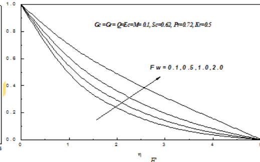
Fig. 12: Effect of the suction parameter ( F_w ) on temperature profiles.
