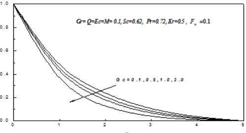
Fig. 20: Effect of the mass Grashof number ( G_c ) on concentration profiles.
