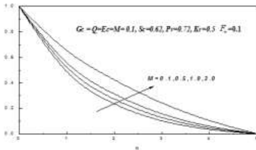
Fig. 9: Effect of the magnetic parameter ( M ) on temperature profiles
