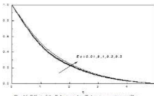
Fig. 15: Effect of the Eckert number ( Ec ) on temperature profiles
