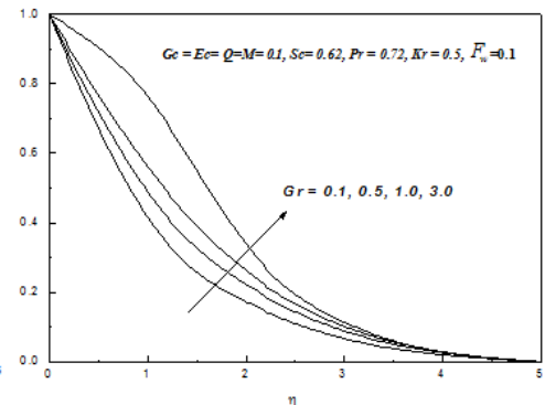
Fig. 2: Effect of the Grashof number ( Gr ) on velocity profiles
