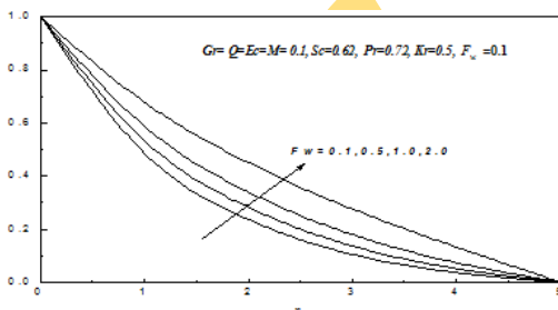
Fig. 21: Effect of the suction ( F_w ) on concentration profiles.
