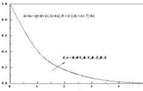
Fig. 7: Effect of the Eckert number ( Ec ) on velocity profiles.
