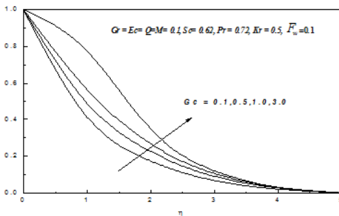
Fig. 3: Effect of the mass Grashof number ( G_c ) on velocity profile
