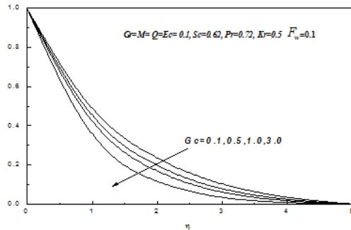
Fig. 11: Effect of the mass Grashof parameter ( Gc ) on temperature profiles.
