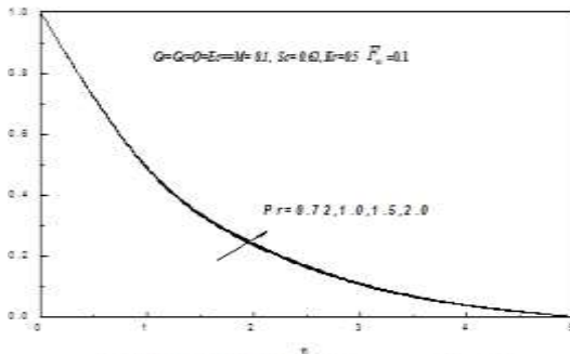
Fig.25: Effect of the Prandtl number ( Pr ) on concentration profiles.
