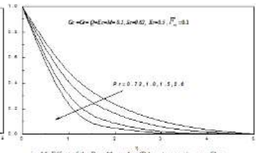
Fig. 16: Effect of the Prandtl number ( Pr ) on temperature profiles
