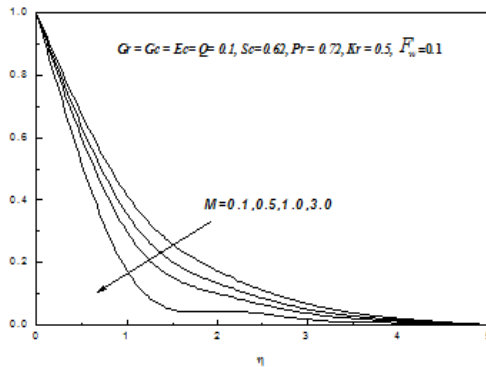
Fig. 1: Effect of the magnetic parameter ( M ) on velocity profiles.
