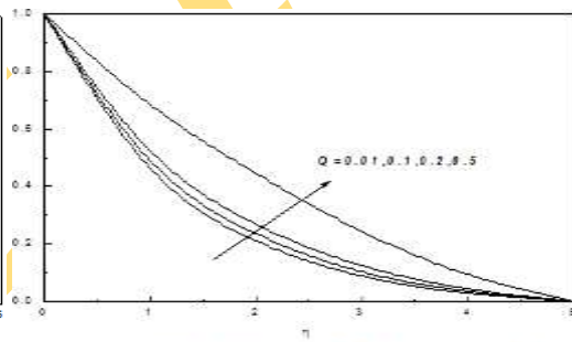
Fig. 14: Effect of the heat generation parameter ( Q ) on temperature profiles.
